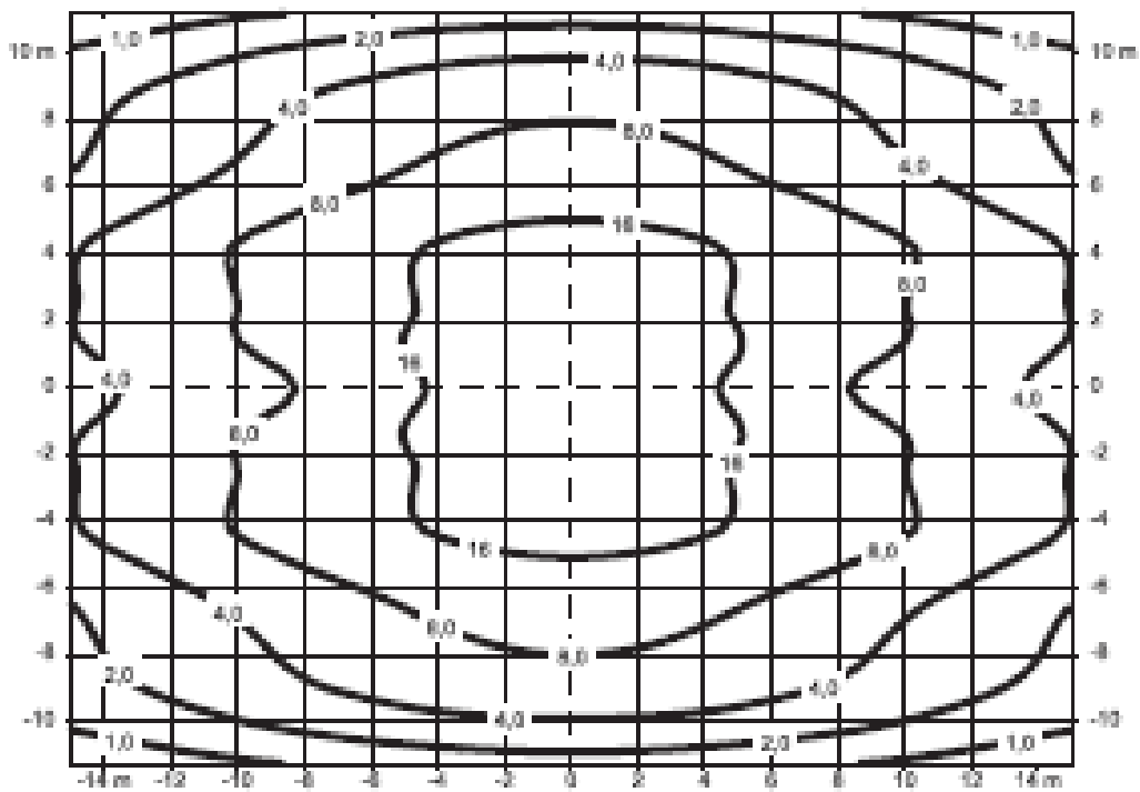
Isolux Diagram
